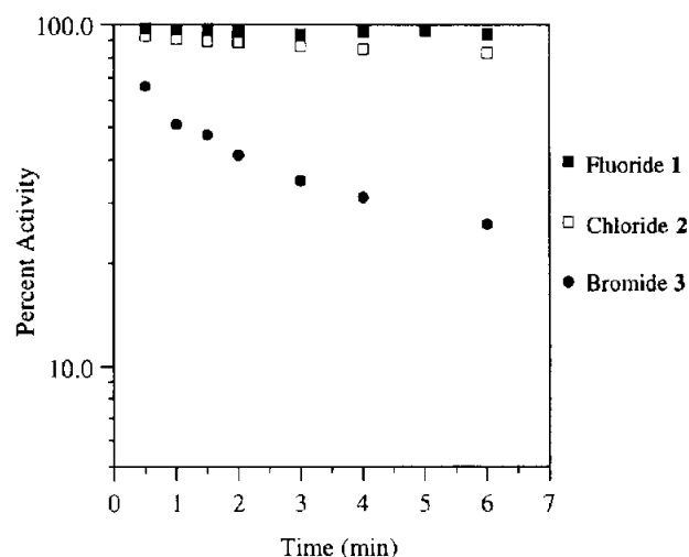
Figure 1. Comparison of the series of \alpha -halobenzylphosphonates as inactivators of Yop51* \Delta 162. Residual enzyme activity following incubation with 5 mM fluoride 1 (■), chloride 2 (□), or bromide 3 (●).
