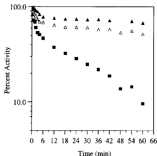
Figure 4. Inactivation of Yop51* \Delta 162 by \alpha -bromobenzylphosphonate is slowed by the presence of substrate. Residual enzyme activity following incubation with 2.5 mM bromide 3 and 0 mM (■), 2 mM ( \Delta ), or 4 mM p -nitrophenylphosphate ( \blacktriangle ).
