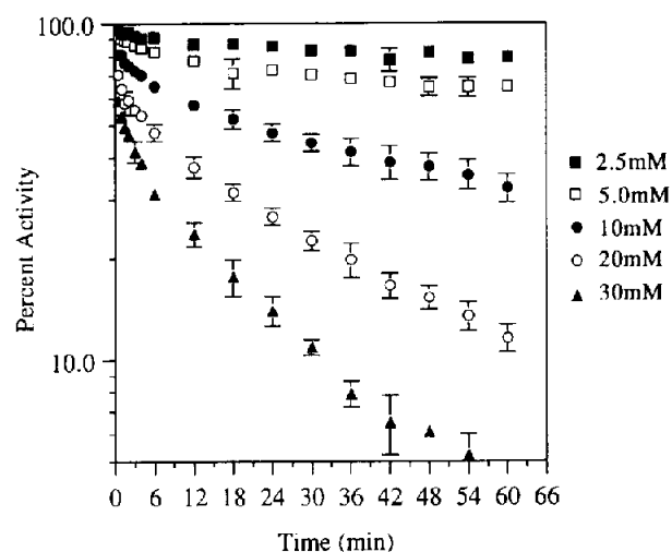
Figure 2. Time-dependent and concentration-dependent inactivation of Yop51* \Delta 162 by \alpha -chlorobenzylphosphonate. Residual enzyme activity following incubation with chloride 2: 2.5 mM (■), 5.0 mM (□), 10.0 mM (●), 20.0 mM (○), and 30.0 mM (closed triangles). Error bars represent the standard deviation of three separate inactivations. In many cases the error bars are smaller than the symbol used to represent remaining activity.
