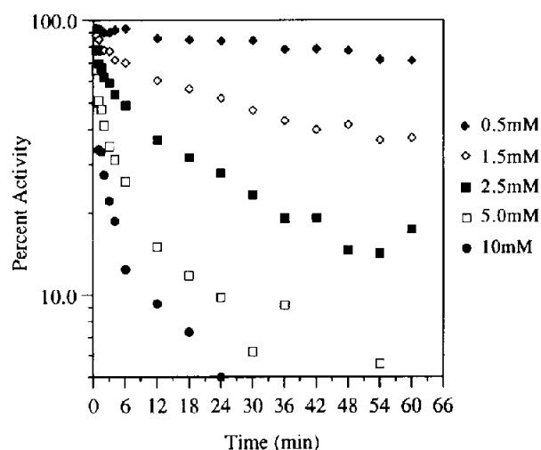
Figure 3. Time-dependent and concentration-dependent inactivation of Yop51* \Delta 162 by \alpha -bromobenzylphosphonate. Residual enzyme activity following incubation with bromide 3: 0.5 mM (◆), 1.5 mM (◇), 2.5 mM (■), 5.0 mM (□), and 10.0 mM (●).
