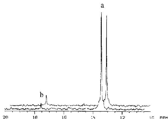
Figure 5. 31 P NMR spectra of the reaction of \alpha -bromobenzylphosphonate and sodium azide. Spectra taken at 10 min (foreground) and 600 min (background) show only bromide 3 (signal a, 13.1 ppm) and solvolysis product (signal b, 17.4 ppm).
