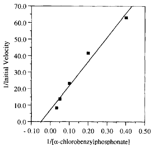
Figure 6. Kitz-Wilson analysis of the inactivation of Yop51 \Delta 162 by \alpha -chlorobenzylphosphonate. Initial velocities were determined from a graph of the natural logarithm of the fractional activities with respect to time for the first 4 min of the inactivation shown in Figure 2.
